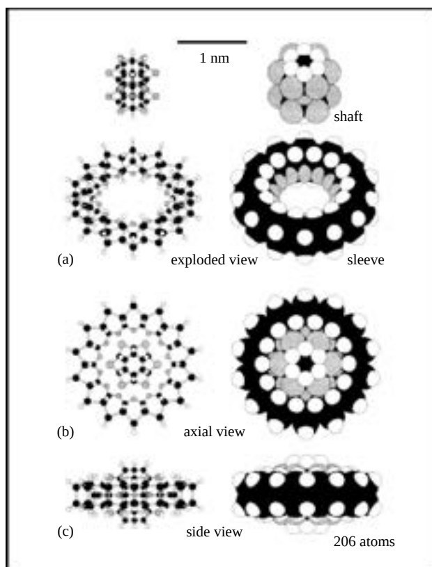
Fig. 3. End views and exploded views of a 206-atom overlap-repulsion bearing. 126 Image courtesy of K. Eric Drexler. © 1992, John Wiley & Sons, Inc. Used with permission.
