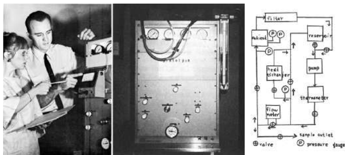
From left: Linda and Fred Chamberlain with perfusion machine Fred designed; machine, front view, the "prototype" shown at the conference; block diagram.
