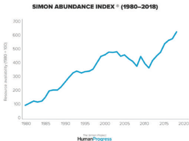
Figure 4: The Simon Abundance Index (1980-2020)
